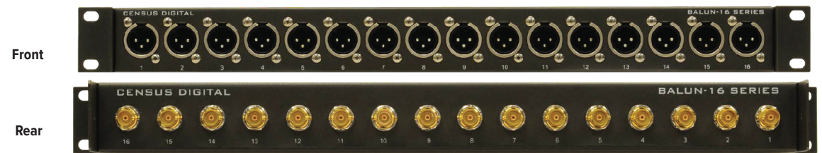
BALUN-16M Impedance Matching Panel 16 XLR Male to 16 BNC
