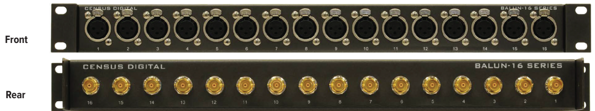
BALUN-16F Impedance Matching Panel 16 XLR Female to 16 BNC
