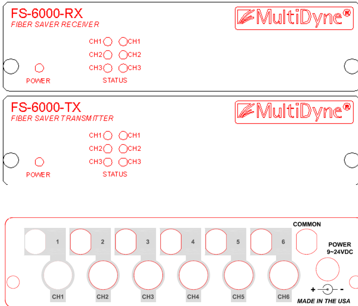
Fig. 1: FTX and FRX front panels, common rear panel
