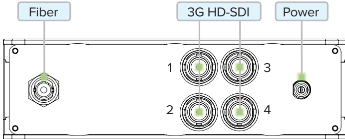
Rear Panel of VB-3607
