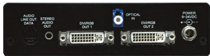
Receiver Rear Panel
